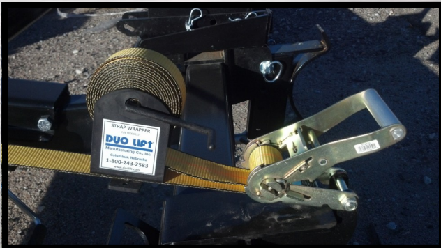
SLIDE Wound Strap Wrapper onto Secured Strap
